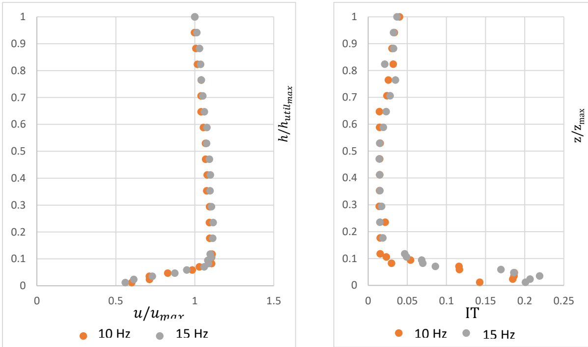
Profil viteza si intensitate turbulenta masurate in zona amonte TA al UTCB in august 2019.
